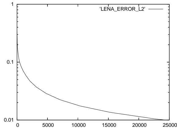
Figure 19: Convergence of the adaptive hp -FEM algorithm. Horizontal and vertical axes represent the number of DOF and the relative error in semi-logarithmic scale, respectively. The algorithm stopped after achieving a relative error of 1%.
