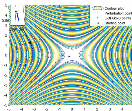
Fig. 5.4. Minimization process of the Schaffer 2 function: Global minimizer x^* = (0,0) with global minimum f(x^*) = 0 .
