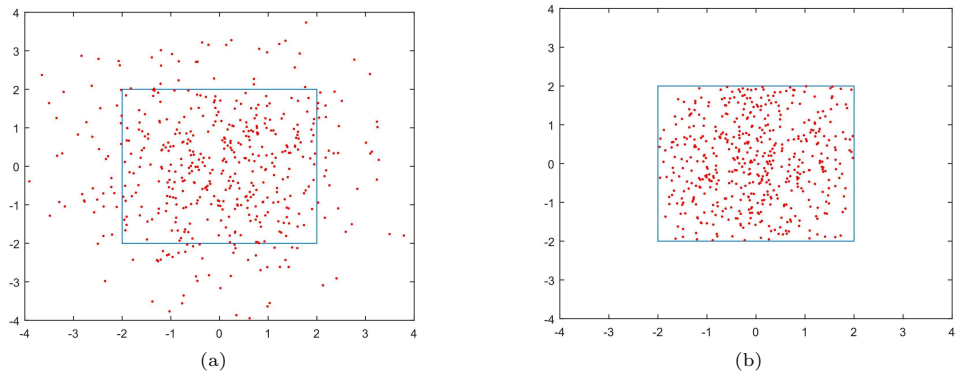
Fig. 4.2. Illustration of 500 points generated by double exponential (a) and our truncated double exponential (b) distributions with \sigma = 2 and \mu = (0, 0) in the box [-2, 2]^2 .
