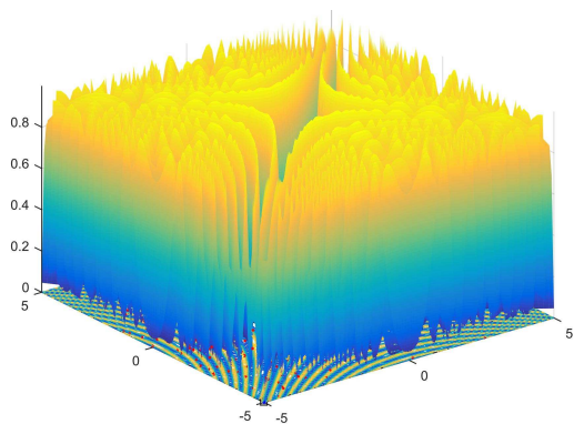
Fig. 5.4. Minimization process of the Schaffer 2 function: Global minimizer x^* = (0,0) with global minimum f(x^*) = 0 .
