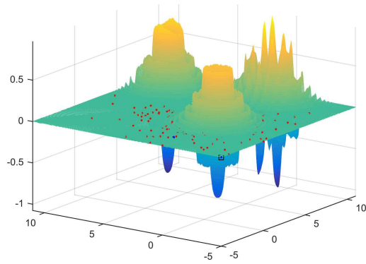
Fig. 5.2. Minimization process of the Modified Langerman function: Global minimizer x^* = (9.68107, 0.66665) with global minimum f(x^*) = -0.96500 .
