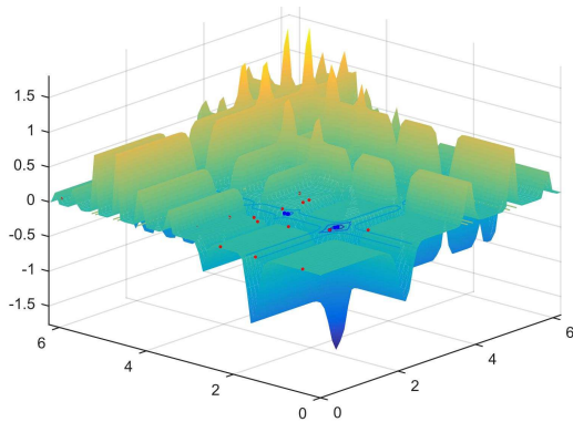
Fig. 5.3. Minimization process of the Michalewicz's function: Global minimizer x^* = (2.2029, 1.5707) with global minimum f(x^*) = -1.8013 .
