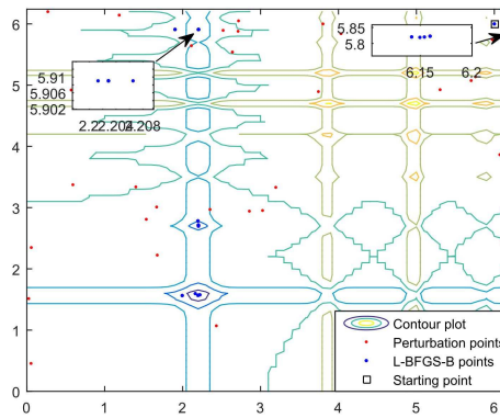
Fig. 5.3. Minimization process of the Michalewicz's function: Global minimizer x^* = (2.2029, 1.5707) with global minimum f(x^*) = -1.8013 .
