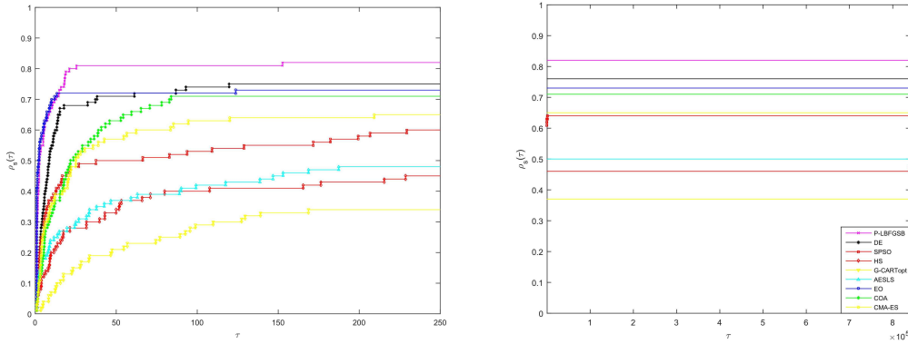
Fig. 7.2. Performance profiles plot based on CPU-time.
