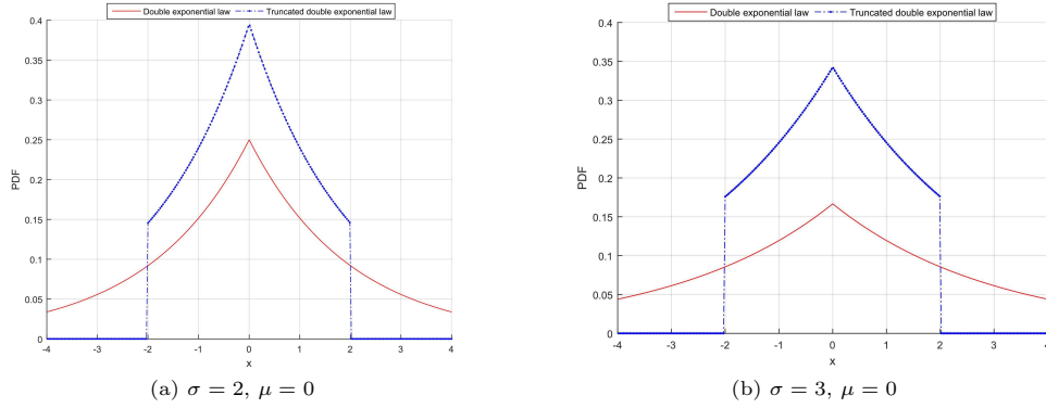
Fig. 4.1. Probability density functions on [-2, 2] , with different diversity parameters.
