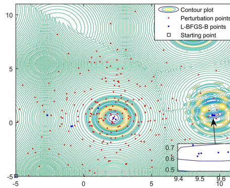
Fig. 5.2. Minimization process of the Modified Langerman function: Global minimizer x^* = (9.68107, 0.66665) with global minimum f(x^*) = -0.96500 .
