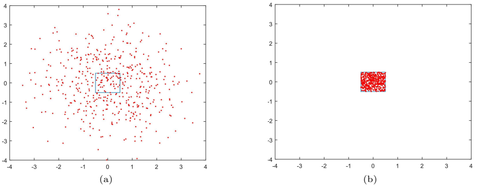
Fig. 4.3. Illustration of 500 points generated by double exponential (a) and our truncated double exponential (b) distributions with \sigma = 2 and \mu = (0, 0) in the box [-0.5, 0.5]^2 .
