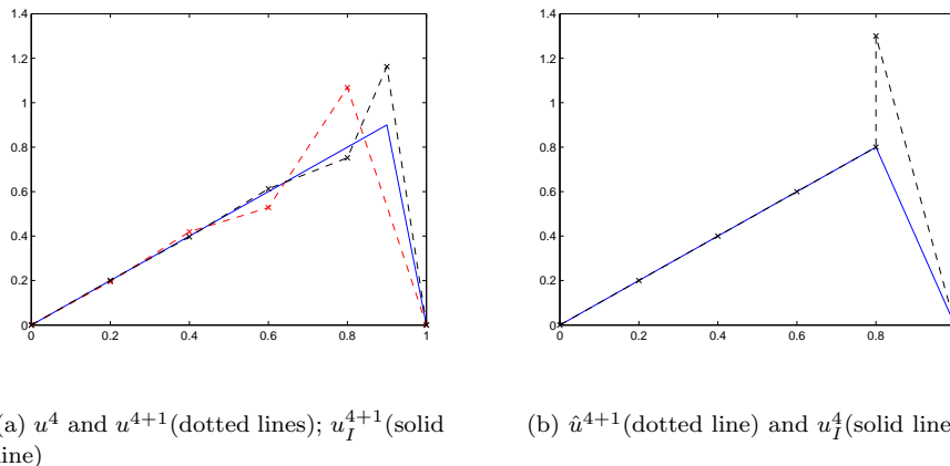
FIGURE 3. FEMs with \varepsilon = 10^{-10} for Example 5.2.
