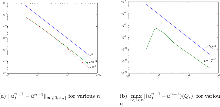
FIGURE 2. Convergence curves with \varepsilon = 10^{-5} and \varepsilon = 10^{-10} for Example 5.1
