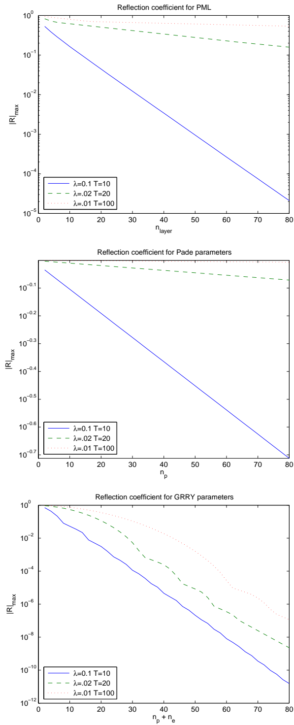
Fig. 5.1. Maximum reflection coefficients for various local domain truncation techniques.
