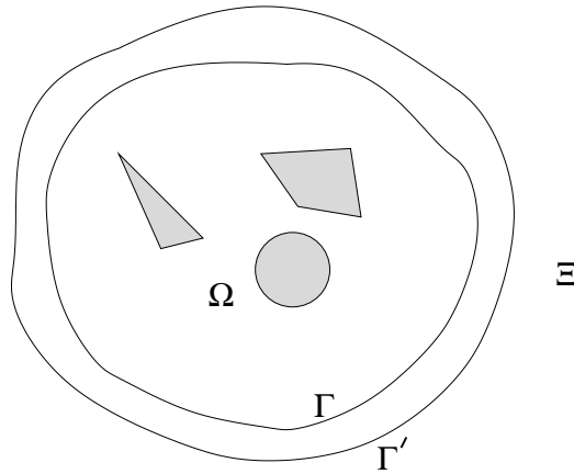
Fig. 3.1. DOMAINS FOR AN EXTERIOR PROBLEM. \Xi is the tail, \Omega is the computational domain, and both \Gamma and \Gamma' are artificial boundaries. The irregular objects within \Omega represent scatterers.
