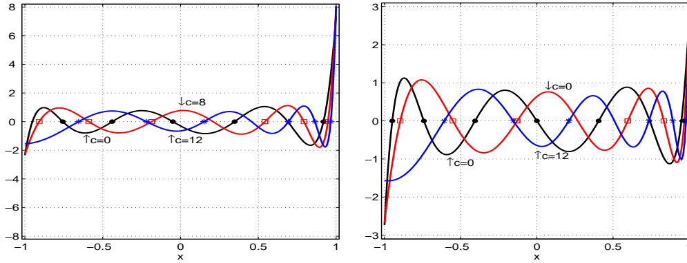
Figure 1: Graph of \varphi_7^{(\alpha)}(x; c) with c = 0, 8, 12 . Left: \alpha = 0.5 . Right: \alpha = 0 .
