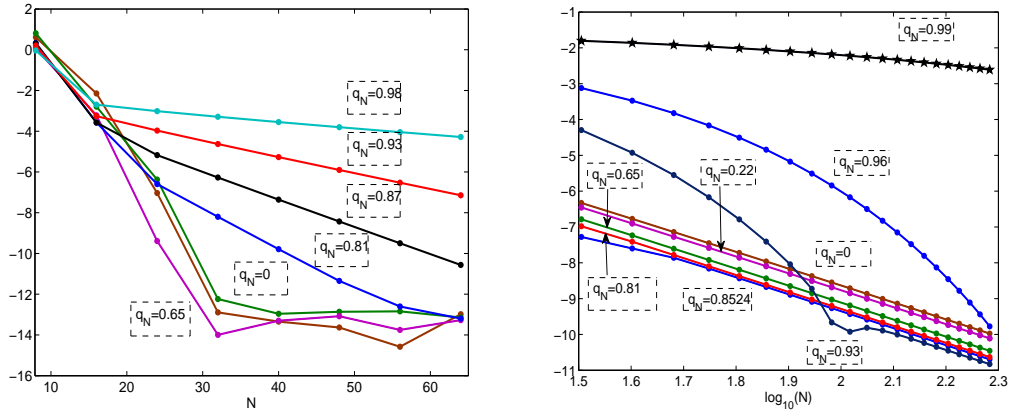
Figure 3: Left (Example 1): \log_{10}(|\hat{u}_N^{(\alpha)}|) against N \in [8, 64] with \alpha = 0 and q_N = 0, 0.22, 0.65, 0.81, 0.87, 0.93, 0.98 . Correspondingly, we have c = \kappa N with \kappa = 0, 0.5, 1, 1.2, 1.3, 1.4, 1.5 . Right (Example 2 with \alpha = 1 ): \log_{10}(|\hat{u}_N^{(\alpha)}|) against \log_{10}(N) with \alpha = 0.5 and q_N = 0, 0.22, 0.65, 0.81, 0.8524, 0.93, 0.96, 0.99 . Correspondingly, c \approx \kappa N with \kappa = 0, 0.5, 1, 1.2, 1.268, 1.4, 1.47, 1.56 .
