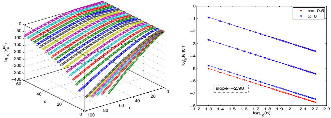
Figure 2: Left: Profiles of \log_{10}(v_n^{(\alpha)}) for various n \in [0, 100] and c \in (0, 60] with \alpha = 0.5 . Right: Decay of the error: \log_{10}(\max_{|k| \leq 1} |\beta_{n+k}^n - \hat{\beta}_{n+k}^n|/c^2) with n \in [20, 160] , c = 1, 5, 10 and \alpha = -0.5, 0 .
