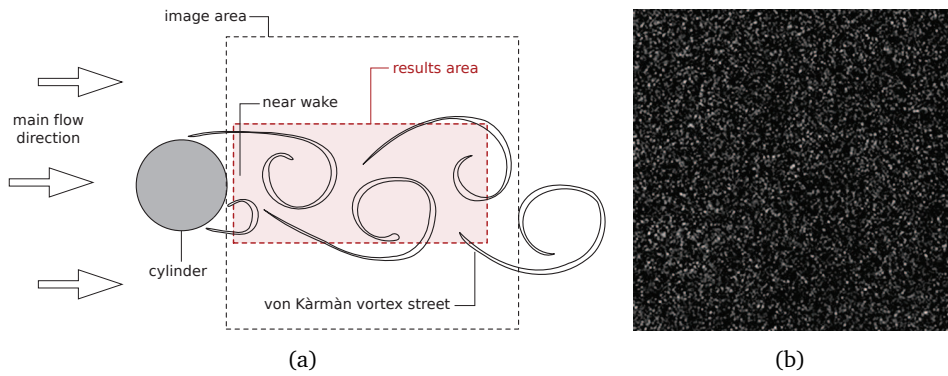
Figure 10: Configuration of the cylinder wake experiment (a); a 256 \times 256 pixels subregion (1/16 of the total area) of a sample of PIV image (b).
