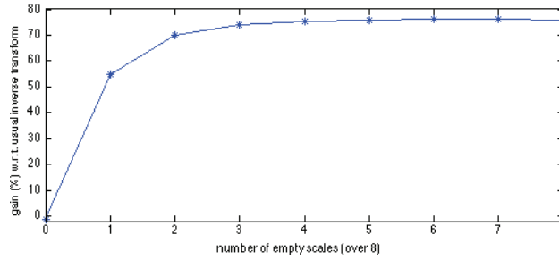
Figure 1: Typical gain observed by the use of a modified filter bank, to save computations by excluding null-coefficient scales. When one scale only is empty, the observed gain is \simeq 55\% , below the theoretical 62.5%.
