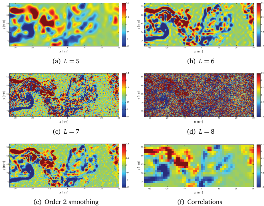
Figure 11: Vorticity comparison. Estimates (a), (b), (c), (d) are obtained with proposed estimator, varying parameter L . Motion (e) is obtained with a more evolved estimator featuring explicit smoothing terms [10]. Last estimate (f) is a reference given by the correlation-based method.
