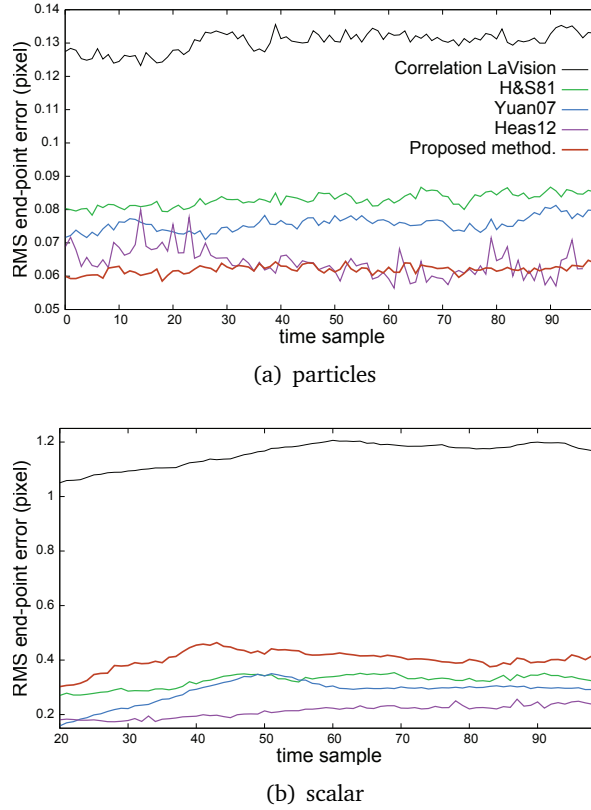
Figure 9: The two sequences introduced in Section 5.1 are processed with parameters (L, C) = (6, 5) and n = 20 for particles, (L, C) = (5, 5) and n = 5 for scalar images. Results (in thick brown ) are compared, in terms of RMSE, to those of other estimators from state-of-the-art: correlation ( gray ), first order regularization [9] ( green ), div-curl regularization [16] ( blue ), multiscale regularization [7] ( purple ). (a) shows particles images results, (b) concerns passive scalar advection .
