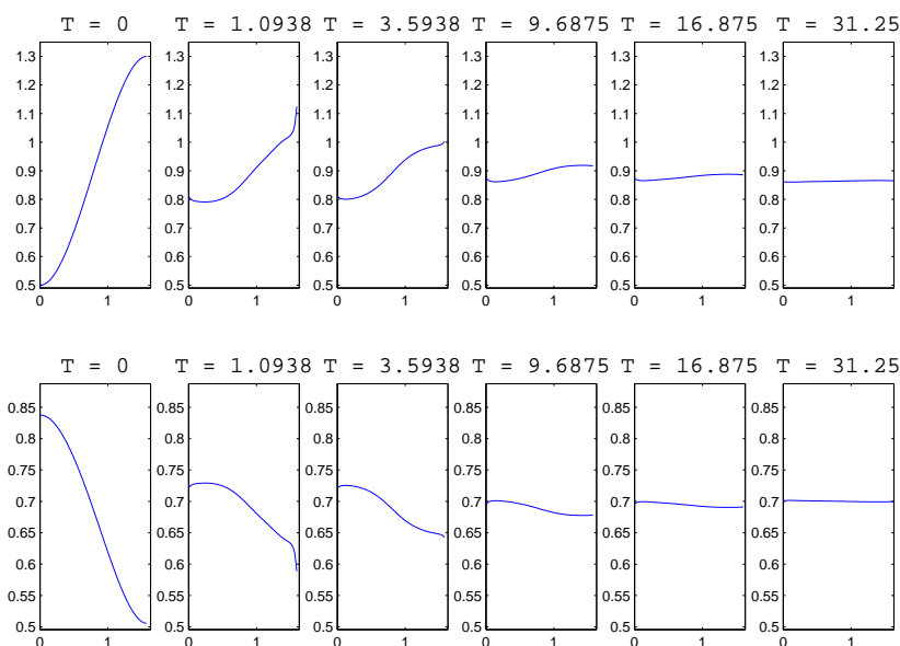
Figure 13: The distribution of the surfactant concentration (top) and the corresponding surface tension (bottom).
