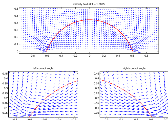
Figure 4: The velocity field for the drop with surfactant near the left and right contact lines ( \eta=0.3, T=1.5625 ).
