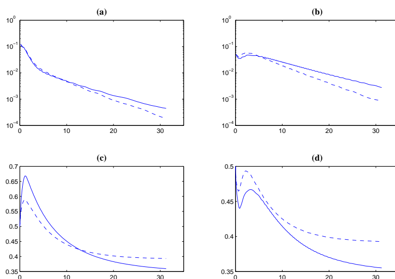
Figure 14: The comparison of a hydrophobic-hydrophilic drop with clean ( \eta=0 , dashed line) and contaminated interface ( \eta=0.3 , solid line). (a) left contact line speed; (b) right contact line speed; (c) left contact angle in units of \pi ; (d) right contact angle in units of \pi .
