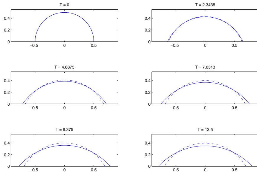
Figure 3: The time evolution of a hydrophilic drop with clean ( \eta=0 , dashed line) and contaminated interface ( \eta=0.3 , solid line).
