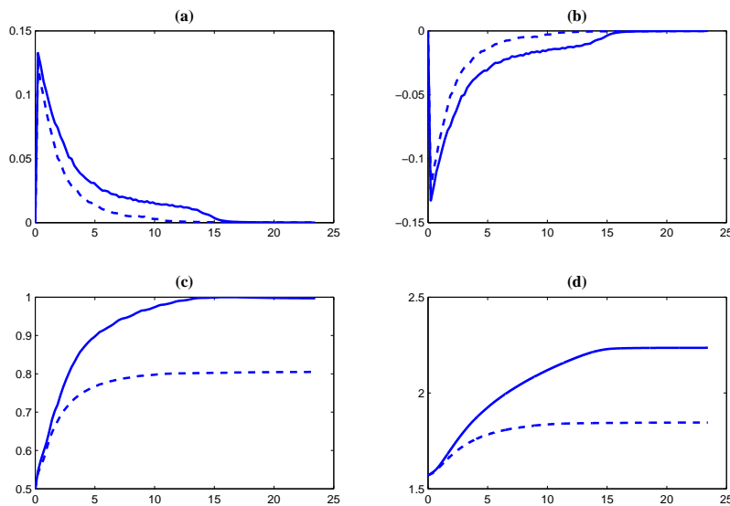
Figure 9: The comparison of a hydrophobic drop with clean ( \eta=0 , dashed line) and contaminated interface ( \eta=0.3 , solid line). (a) left contact line speed; (b) right contact line speed; (c) contact angles in units of \pi ; (d) total length of the drop.
