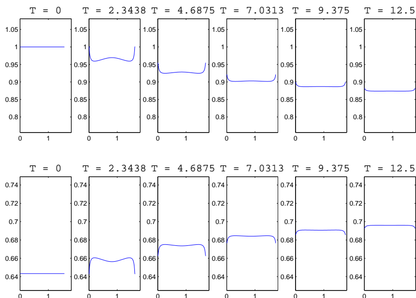
Figure 5: The distribution of the surfactant concentration (top) and the corresponding surface tension (bottom).
