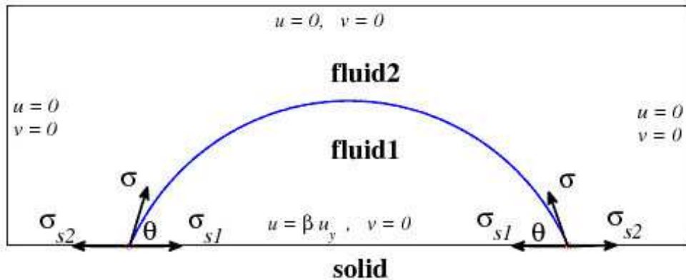
Figure 1: The diagram of contact lines and the problem set up.
