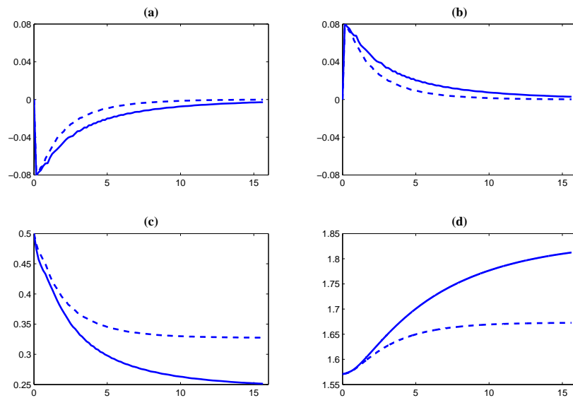
Figure 6: The comparison of a hydrophilic drop with clean ( \eta=0 , dashed line) and contaminated interface ( \eta=0.3 , solid line). (a) left contact line speed; (b) right contact line speed; (c) contact angles in units of \pi ; (d) total length of the drop.
