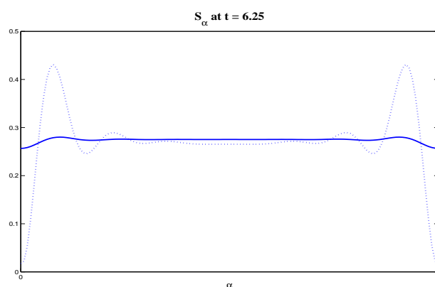
Figure 2: Comparison of stretching factor |\mathbf{X}_\alpha| = S_\alpha with ( U^A = 0 , dotted line) and ( U^A \neq 0 , solid line), where h = 1/128 .
