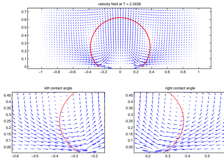
Figure 8: The velocity field for the drop with surfactant near the left and right contact lines ( \eta=0.3, T=2.3438 ).
