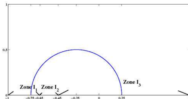
Figure 10: Wettability and the initial drop set up.
