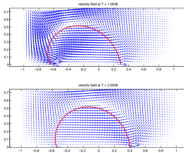
Figure 12: The velocity field for the drop with contaminated interface near the left and right contact lines at T=1.0938 and T=3.5938 .
