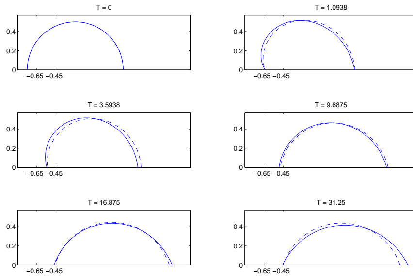
Figure 11: The time evolution of a hydrophobic-hydrophilic drop with clean ( \eta=0 , dashed line) and contaminated interface ( \eta=0.3 , solid line).
