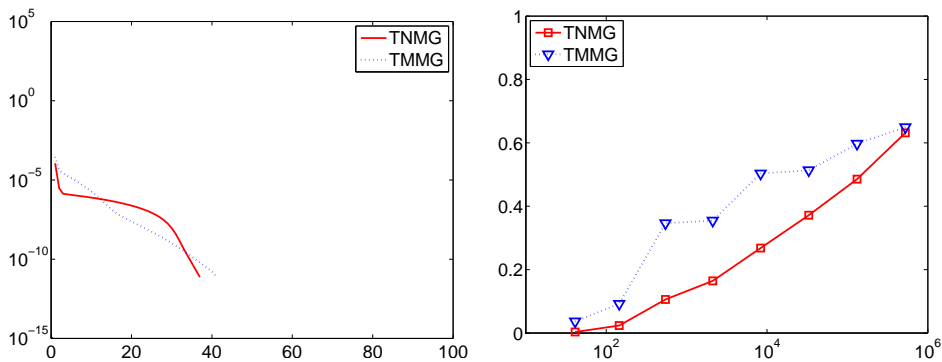
Fig. 7.13. Degenerate Problem: Iteration history for nested iteration (left) and asymptotic convergence rates (right).
