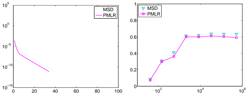
Fig. 7.5. Degenerate problem: Iteration history for nested iteration (left) and asymptotic convergence rates (right).
