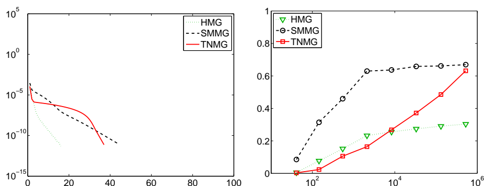
Fig. 7.14. Degenerate Problem: Iteration history for nested iteration (left) and asymptotic convergence rates (right).
