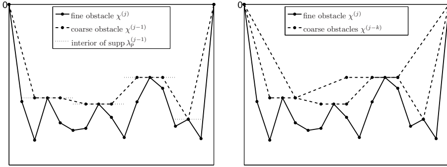
Fig. 4.1. Restriction (left) and hierarchical decomposition (right) of defect obstacle.
