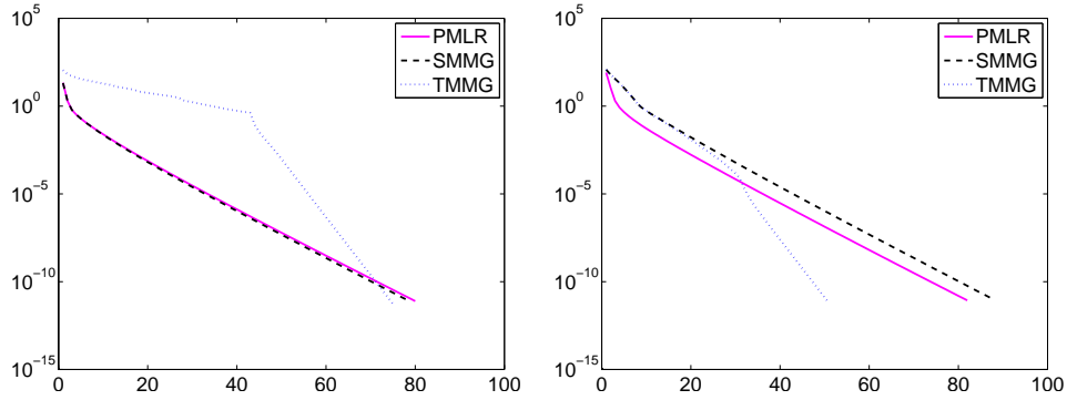
Fig. 7.6. Spiral problem: Iteration histories for the initial iterates u_j^0 = \varphi_j (left) and u_j^0 = \varphi_j + 10 > \varphi_j (right).
