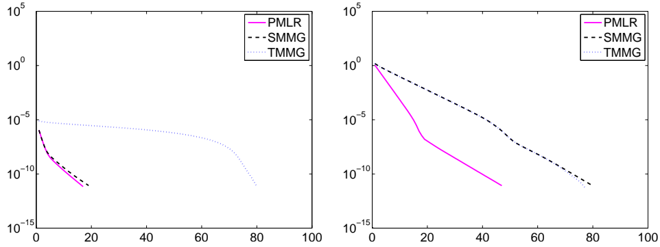
Fig. 7.8. Degenerate Problem: Iteration histories for the initial iterates u_j^0 = \varphi_j (left) and u_j^0 = 0 > \varphi_j (right).
