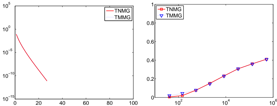
Fig. 7.11. Spiral problem: Iteration history for nested iteration (left) and asymptotic convergence rates (right).
