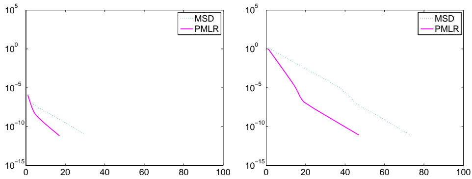
Fig. 7.4. Degenerate problem: Iteration histories for the initial iterates u_j^0 = \varphi_j (left) and u_j^0 = \varphi_j + 10 > \varphi_j (right).
