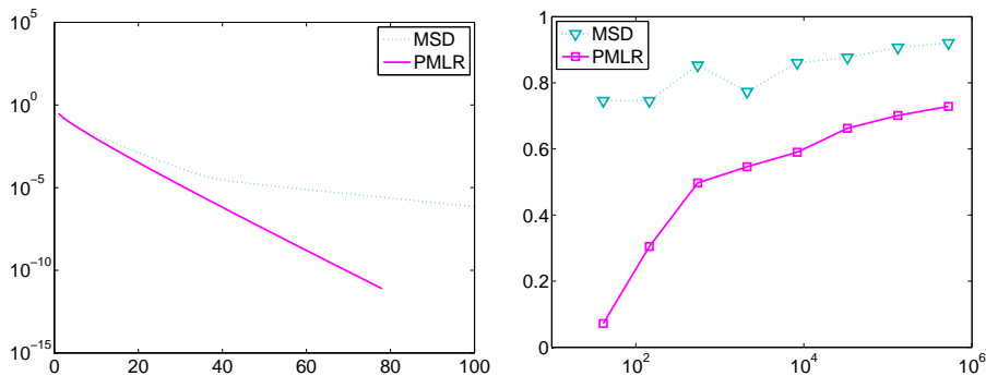
Fig. 7.3. Spiral problem: Iteration history for nested iteration (left) and asymptotic convergence rates (right).
