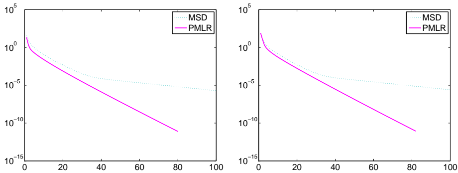
Fig. 7.2. Spiral problem: Iteration histories for the initial iterates u_j^0 = \varphi_j (left) and u_j^0 = \varphi_j + 10 > \varphi_j (right).
