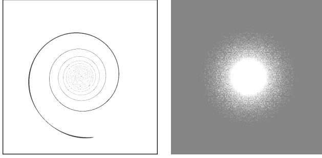
Fig. 7.1. Coincidence sets of spiral problem (left) and degenerate problem (right).
