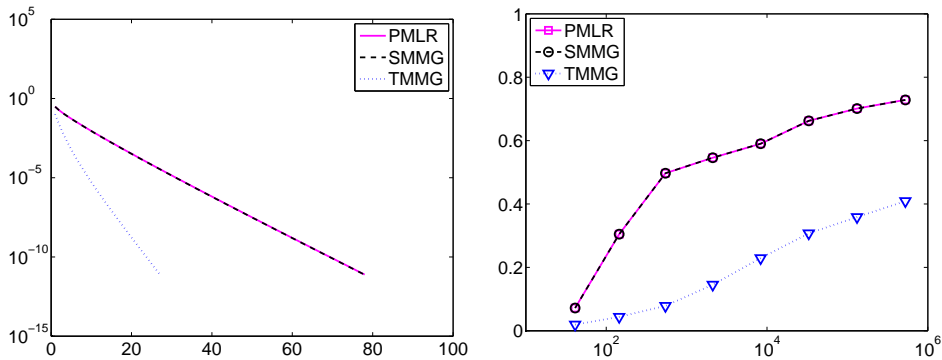
Fig. 7.7. Spiral problem: Iteration history for nested iteration (left) and asymptotic convergence rates (right).
