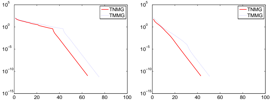
Fig. 7.10. Spiral problem: Iteration histories for the initial iterates u_j^0 = \varphi_j (left) and u_j^0 = 0 > \varphi_j (right).
