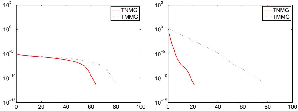
Fig. 7.12. Degenerate Problem: Iteration histories for the initial iterates u_j^0 = \varphi_j (left) and u_j^0 = 0 > \varphi_j (right).
