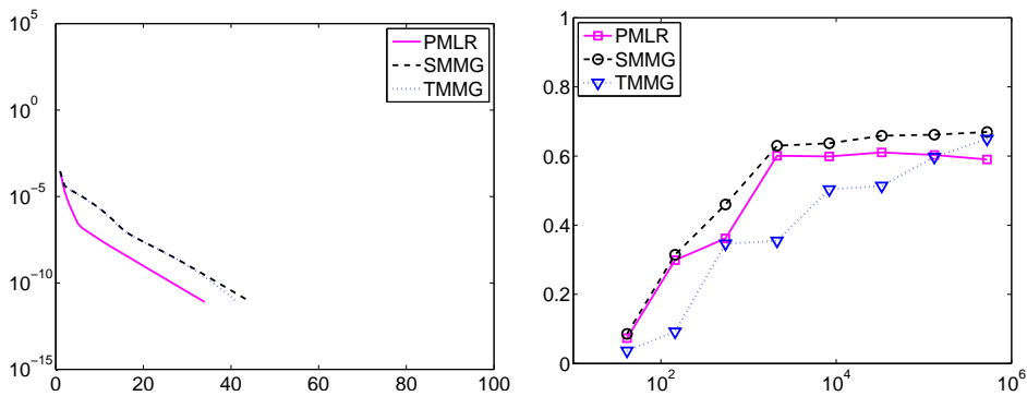
Fig. 7.9. Degenerate Problem: Iteration history for nested iteration (left) and asymptotic convergence rates (right).
