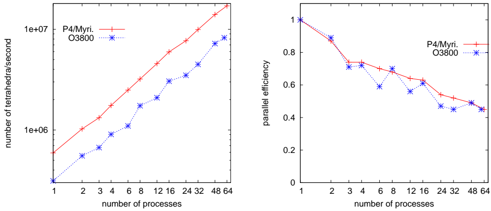
Figure 8: The number of the tetrahedra per second (left) and the parallel efficiency (right) against the number of processes for the first example.
