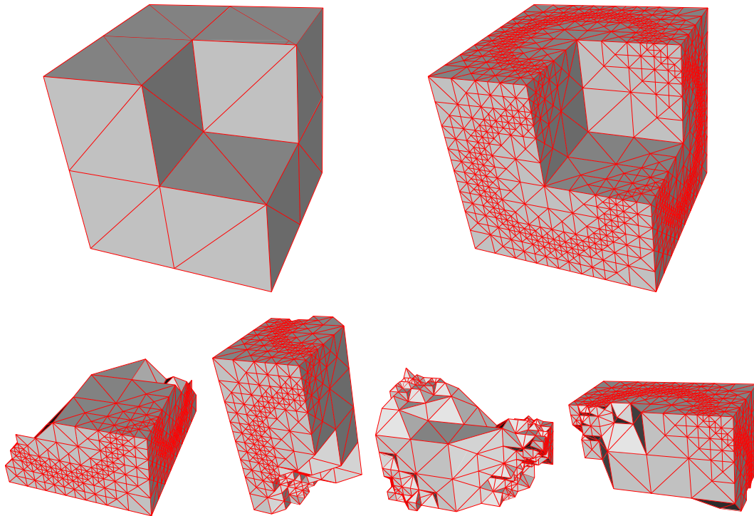
Figure 9: The initial mesh (top left), a refinement mesh with 42,546 tetrahedra (top right) and a partitioned mesh (bottom) for the second example.
