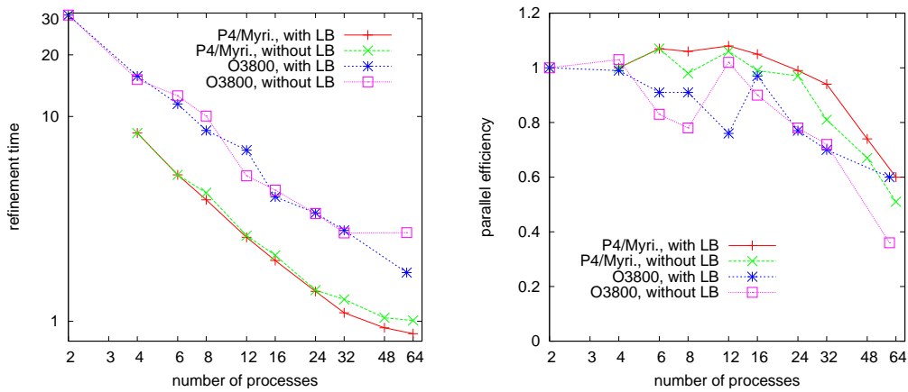
Figure 10: The refinement time (left) and the parallel efficiency (right) against the number of processes for the second example.
