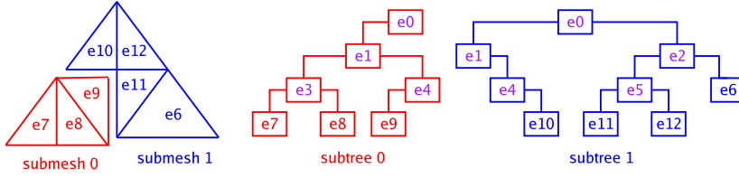
Figure 6: Subtrees for a partitioned mesh.
