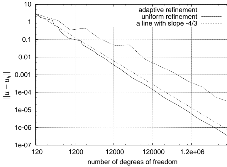
Figure 11: Convergence history of the 4-th order Lagrange element for the third example.
